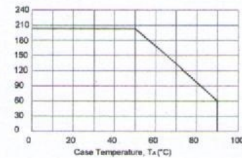
<Fig.a> Forward Current Derating Curve
