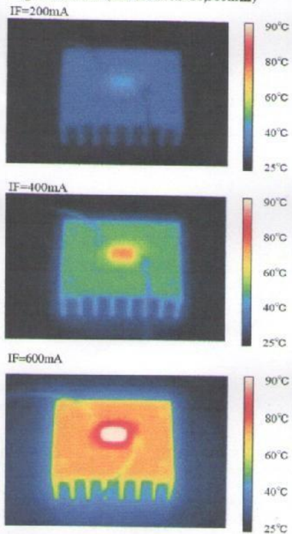
<Fig.2> Board A (surface area=10,300mm 2 )
