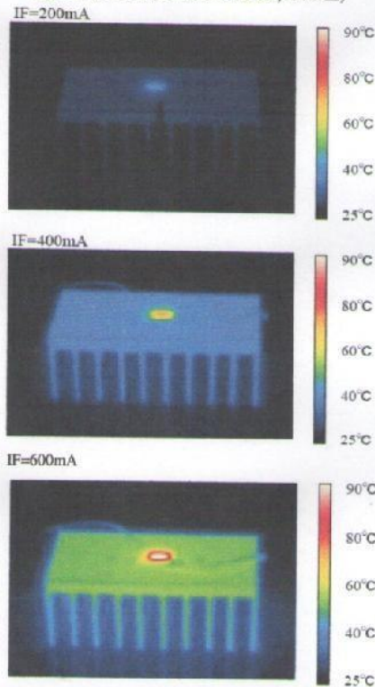
<Fig.3> Board B (surface area=20,600mm 2 )
